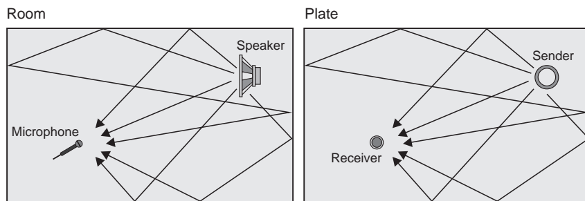
Fig. 4.3: Room reflections and reverb plate reflections
